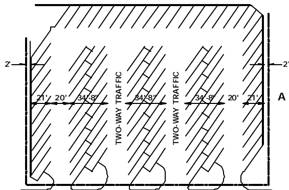
60 Degree Layout with Two-Way Traffic
