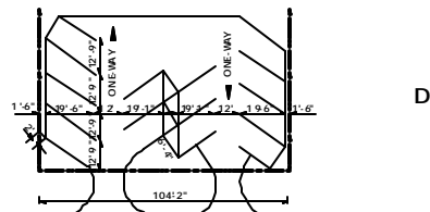
45 Degree Layout with One-Way Traffic
