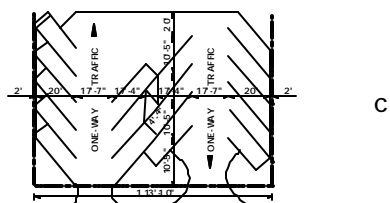
60 Degree Layout with One-Way Traffic
