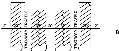
45 Degree Layout with Two-Way Traffic
