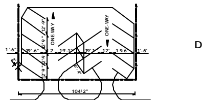
45 Degree Layout with One-Way Traffic
